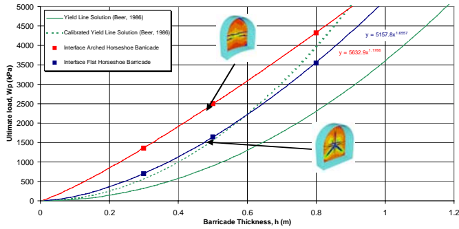
Fig. 19. Ultimate load for shear interface 5 × 5 m flat horseshoe and arched horseshoe, 30 MPa shotcrete bulkheads.
