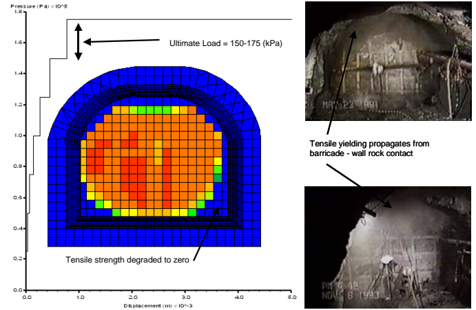
Figure 21. Failure pressure and failure mechanism predicted with FLAC3D compared to in situ pressure tests conducted at the Gaspé Mine (after, Miller et al., 1991).
