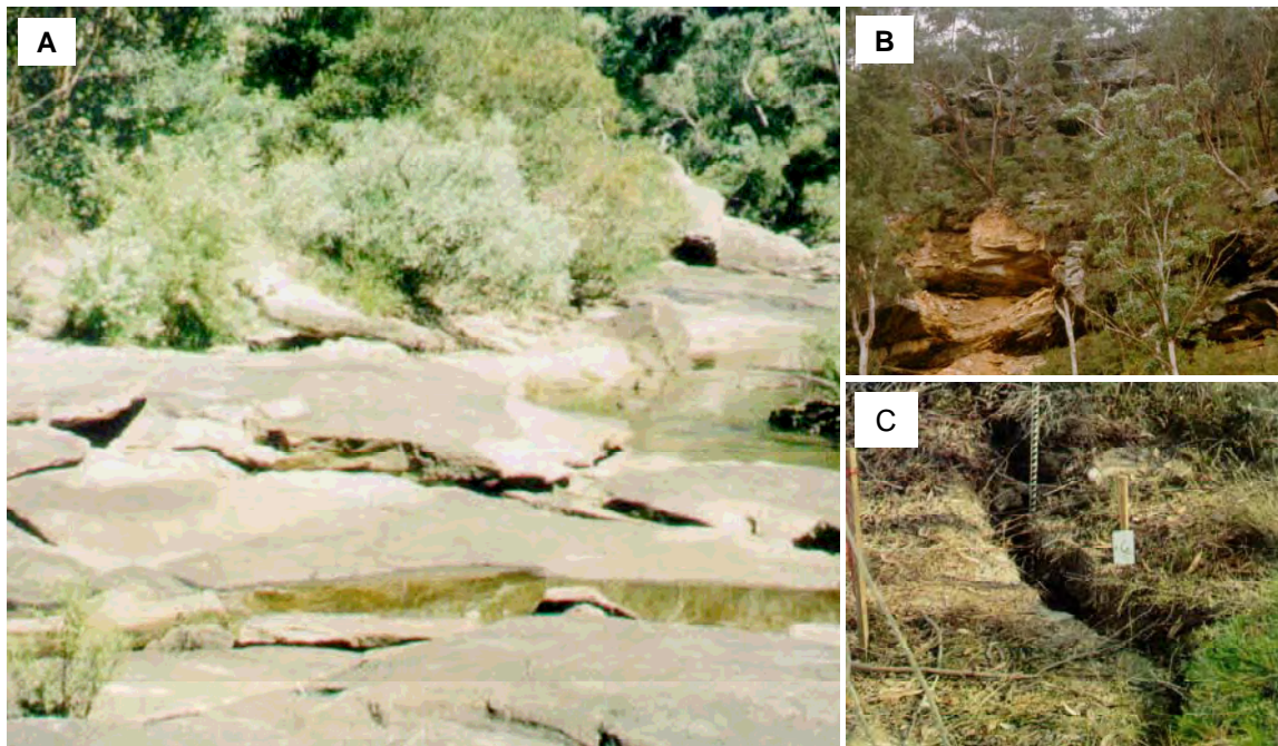
Figure 8 a) Low-angle fractures observed above Panel 8 at the Tower Colliery (after Holla and Barclay, 2000); b) localised rockfall above Longwall 15 (ACARP, 2002); c) tension crack behind escarpment (after Holla and Barclay, 2000)
