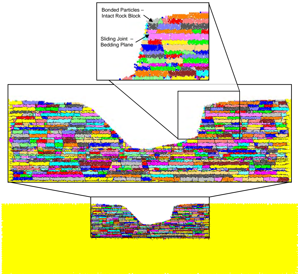
Figure 13 Synthetic rock mass produced to simulate Hawkesbury Sandstone
