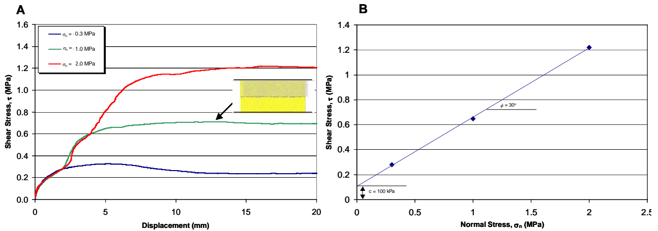
Figure 11 Shear behaviour of sliding joints used to simulate bedding and joint surfaces
