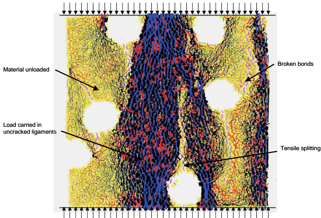
Figure 6 Force distributions and broken bonds in a cemented granular material with six initial holes in the post-peak portion of an unconfined compression test (Potyondy and Cundall, 2004)
