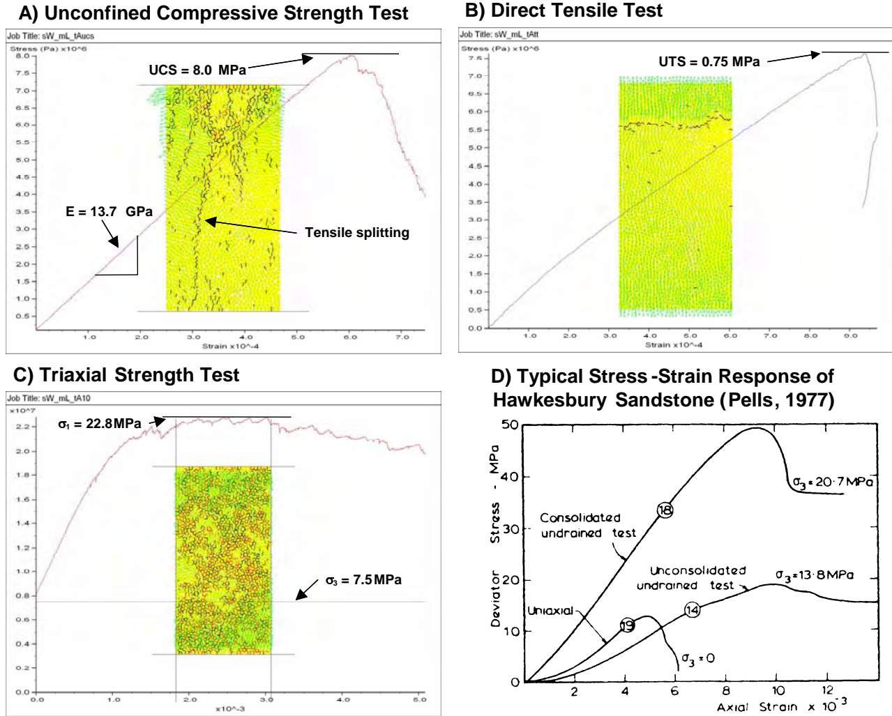
Figure 9 Results of PFC calibration of weak intact Hawkesbury Sandstone
