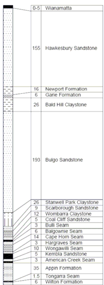
Figure 1 a) Typical stratigraphic column in the Southern Coalfield (after ACARP, 2001); b) typical steep sided river valley formed within the Hawkesbury Sandstone
