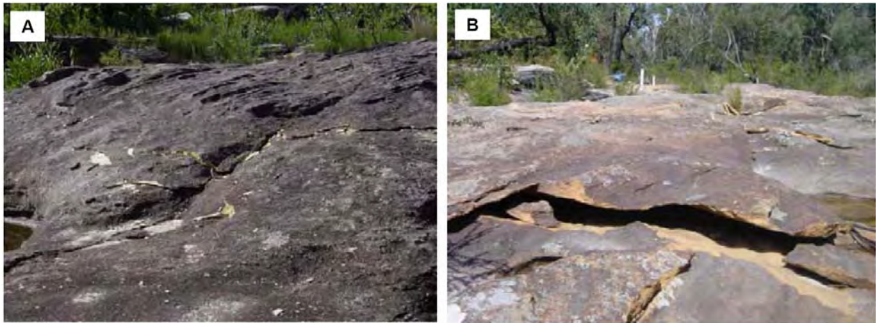
Figure 3 Low-angle shear structures in river beds within the Southern Coalfield
