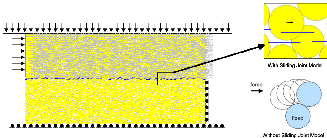
Figure 10 Direct-shear testing environment used to simulate sliding joint macroscopic behaviour
