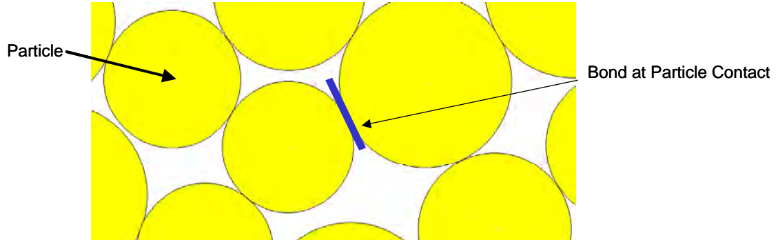
Figure 5 PFC particle and bond geometry
