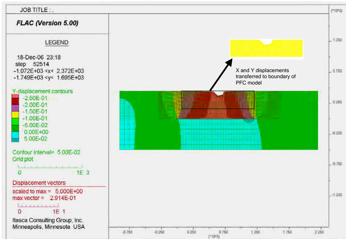
Figure 14 Regional FLAC model used to simulate displacement profile at the boundary of the PFC model
