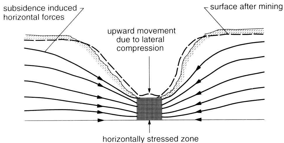
Figure 2 Conceptual model of the upsidence mechanism (after Holla, 1997)
