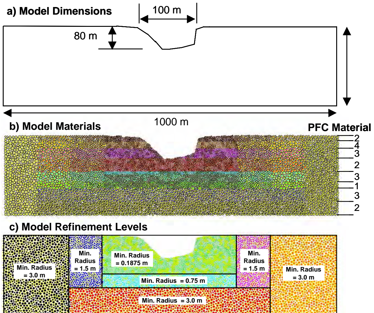
Figure 12 Dimensions, material groups and particle refinement zones of PFC model used to simulate the centreline of Panel 8 at the Tower Colliery
