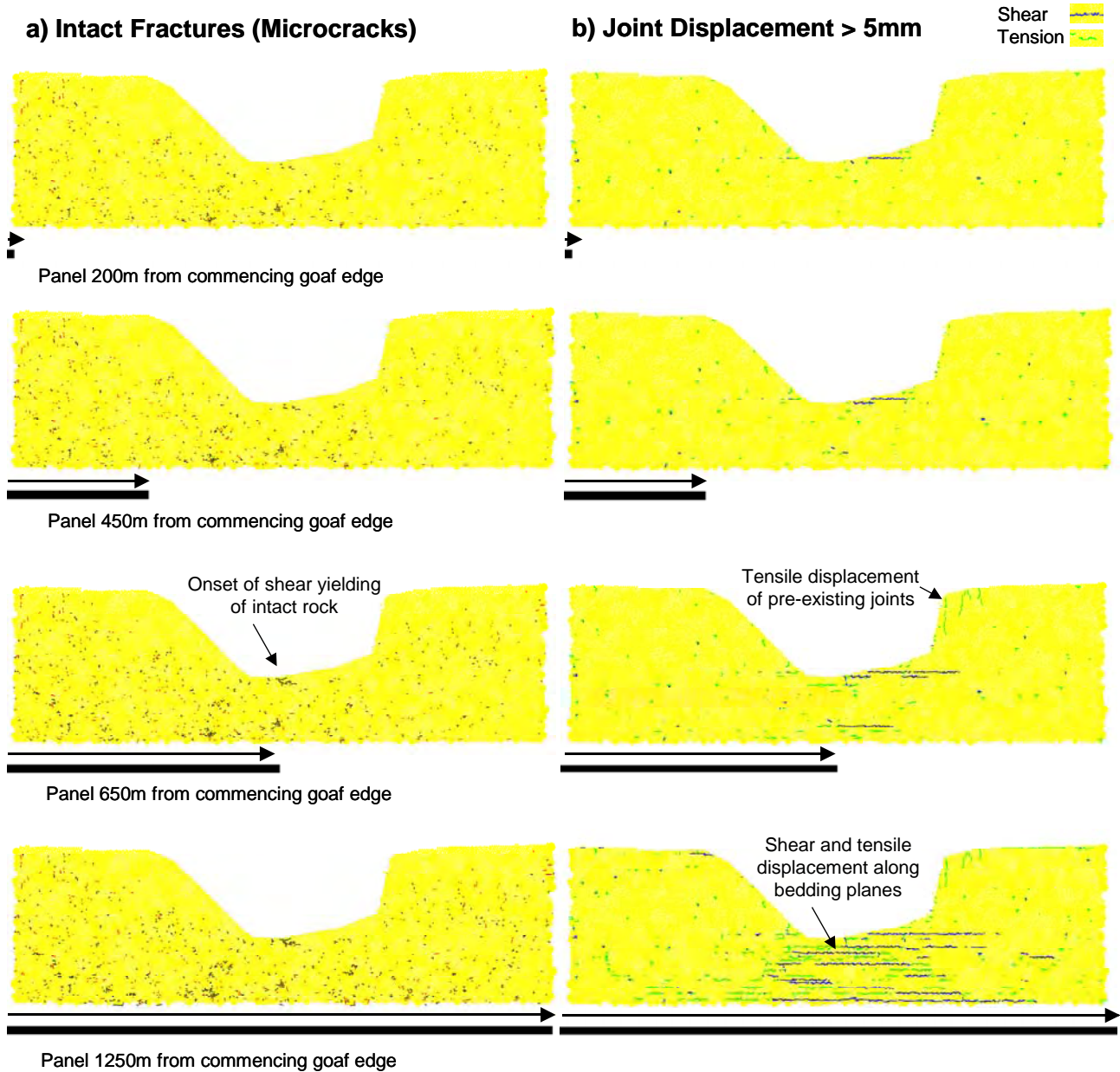
Figure 15 Evolution of fracturing beneath the Cataract Gorge
