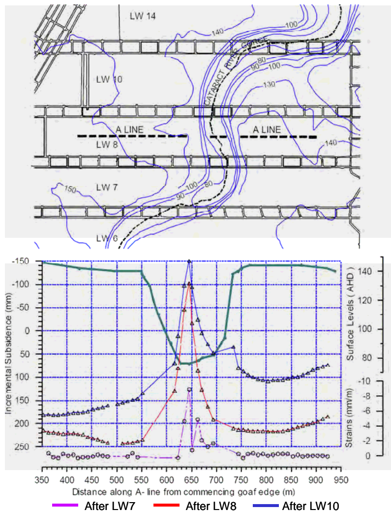
Figure 7 Subsidence monitoring above Panel 8 at the Tower Colliery (after ACARP, 2002)
