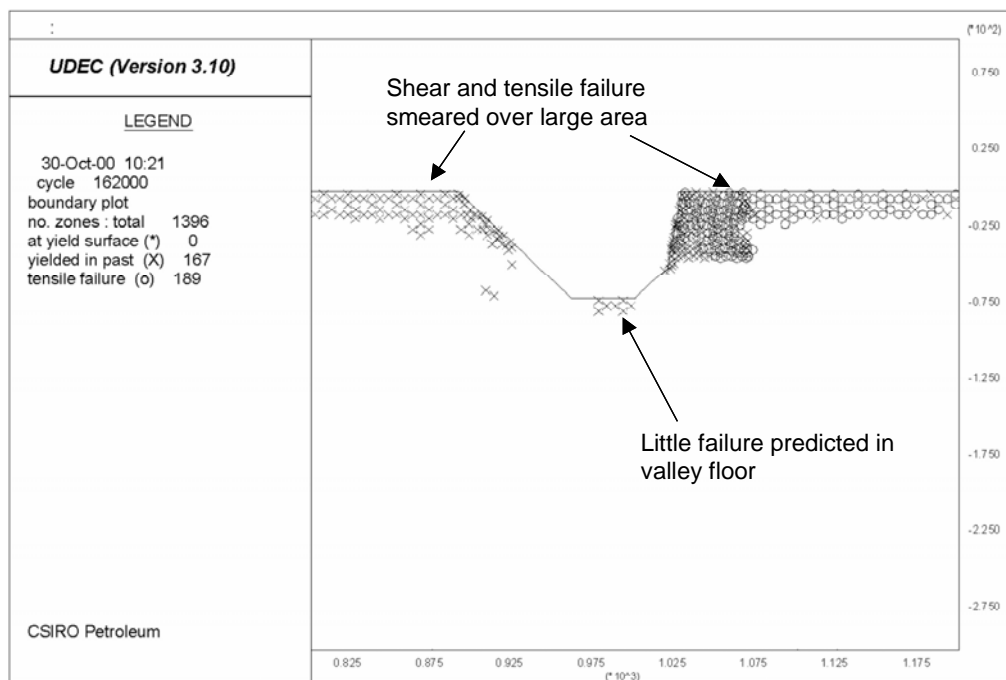
Figure 4 UDEC simulation of longwall mining beneath the Cataract River at Tower Colliery (after ACARP, 2002)
