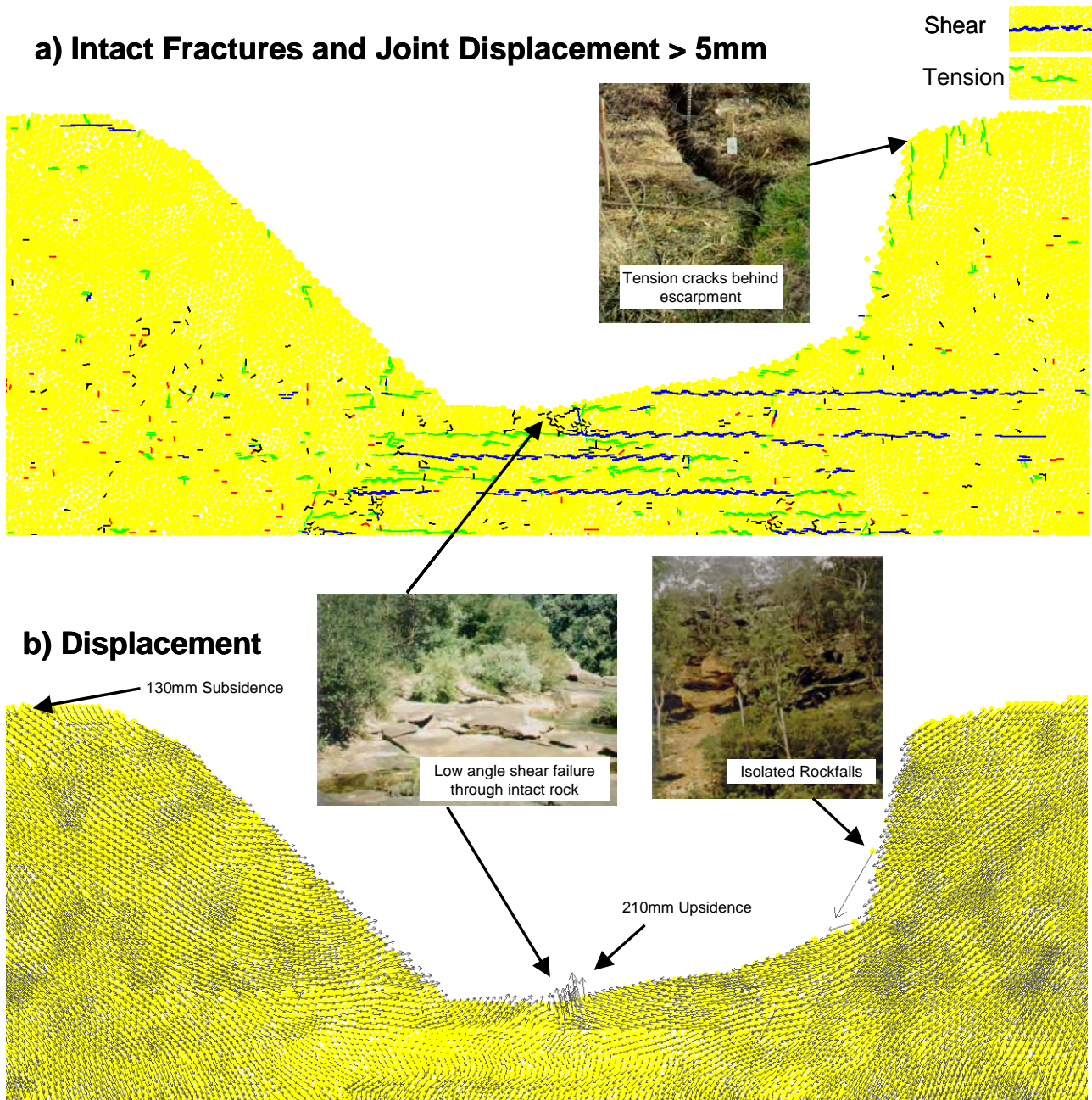
Figure 16 Explicit fracturing and displacement at the base of the Cataract Gorge
