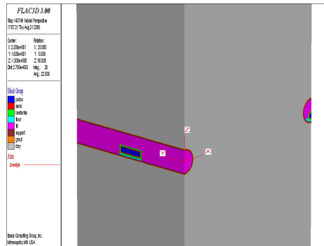
Tunnel (pink) and canister (blue) layout, northern site
